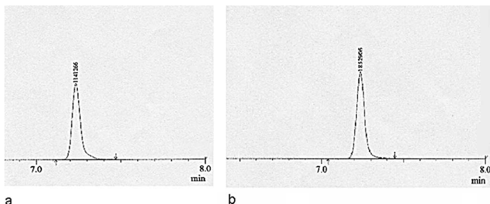
Figure 2. (a) Representative standard toluene gas-chromatographic trace ( 0.60 \mu\text{g l}^{-1} ) and (b) representative toluene gas-chromatographic trace ( 0.97 \mu\text{g l}^{-1} ) in the exhaled breath condensate of a subject after exposure.
